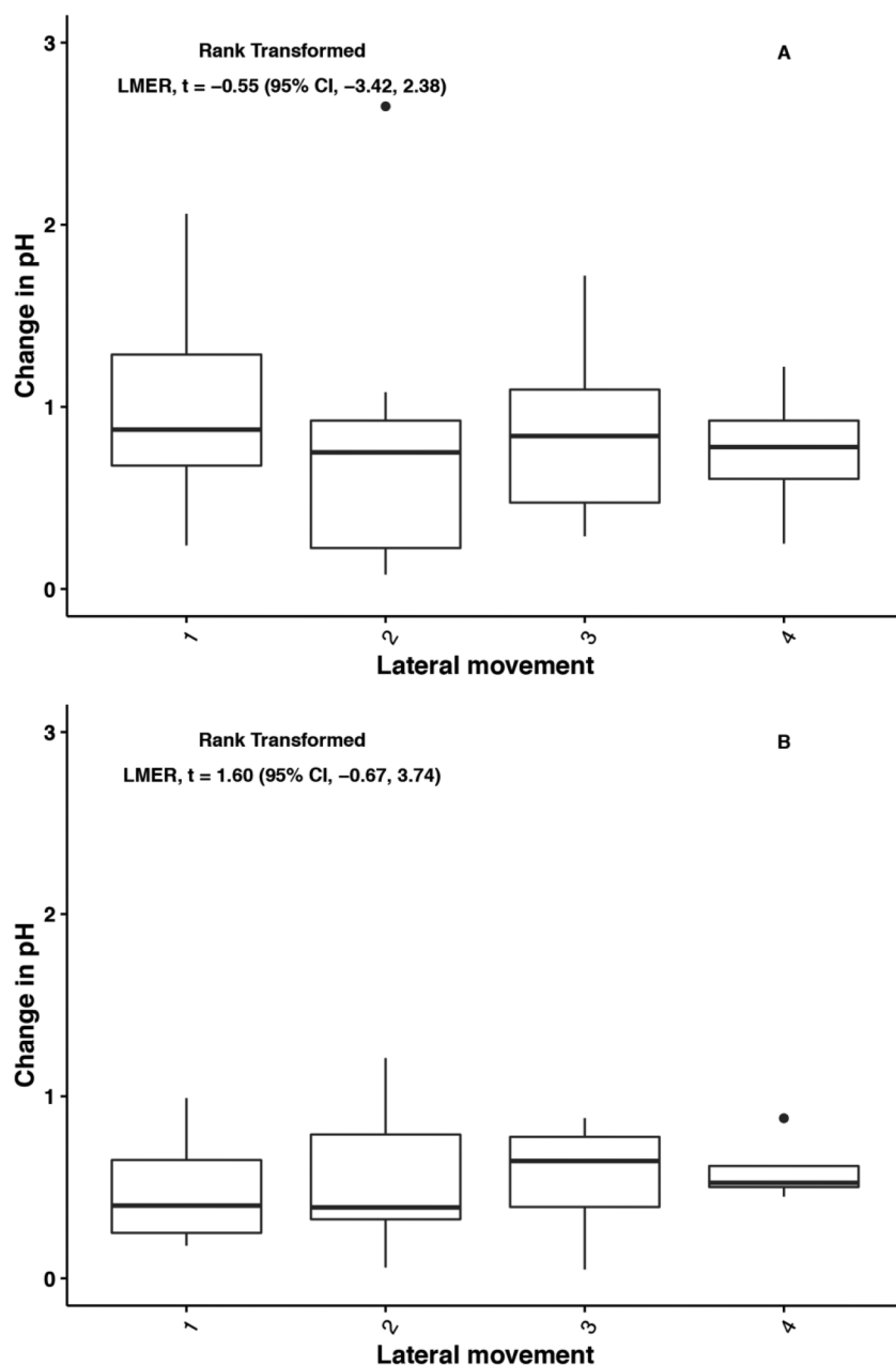
Fig. 6. Boxplots of the change in pH during the first four lateral movements ( \text{CO}_2 vein to no \text{CO}_2 vein) made during trials when a \text{CO}_2 plug was added to the flume (panel A: \text{CO}_2 was added to the inner vein of the flume; panel B: \text{CO}_2 was added to the outer vein of the flume). Thick black lines represent medians (50% quantiles), the box represents the interquartile ranges (IQR; the 25th and 75th quantiles), vertical lines are whiskers and represent the higher and lower 1.5 of the IQR, and black dots represent outlying points. No statistical differences were calculated with a linear mixed effects model using a Gaussian error distribution when change in pH was rank-transformed.
